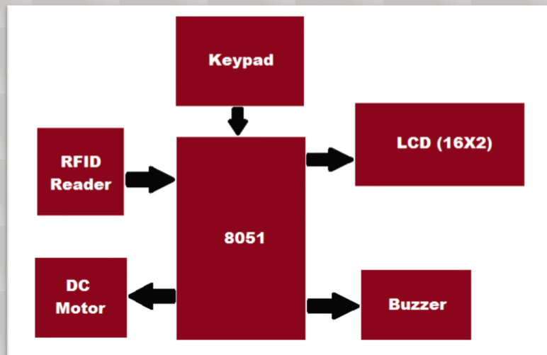
Fig 3. Block diagram of door locking system
