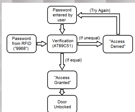
Fig. 5: Flowchart explaining the algorithm
