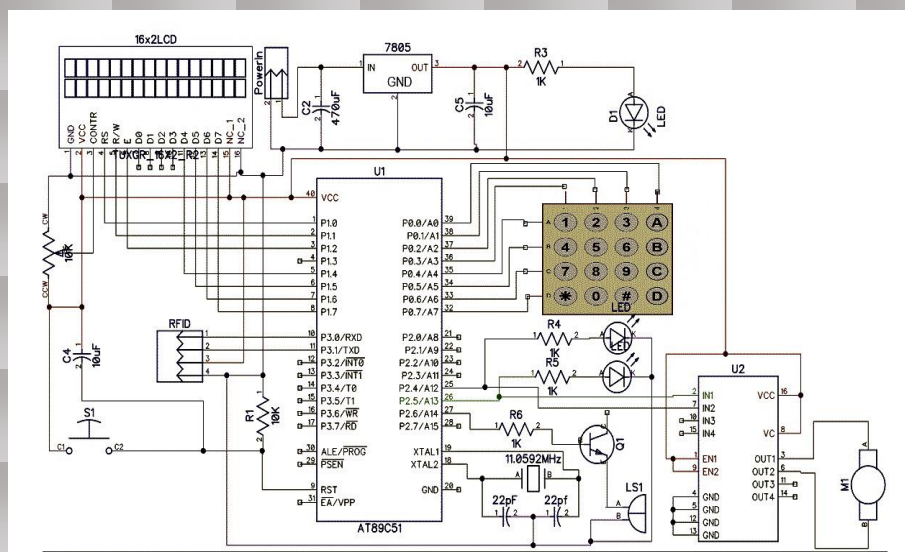
Fig. 4: Circuit Diagram of Door Locking System
