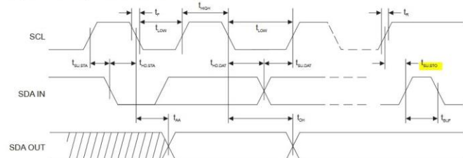
Figure 2-3. I 2 C Synchronous Data Timing
