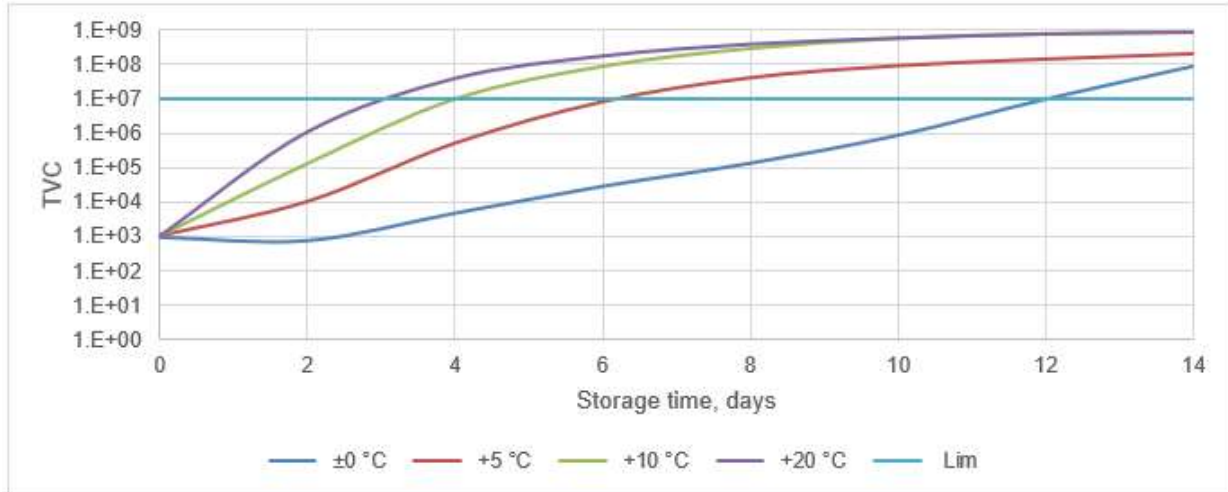
Effect of temperature on the shelf life of meat. TVC - the number of bacteria per cm 2
