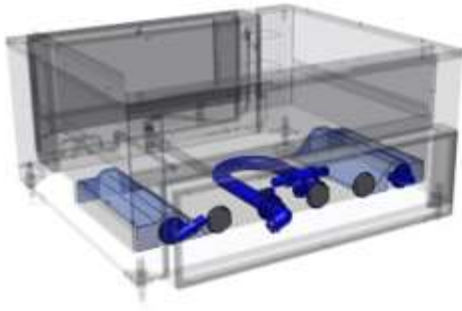
Water supply and drain elements of the Chilling Tank
